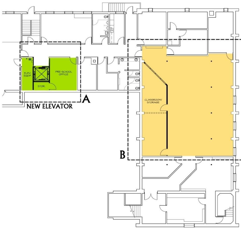
BASEMENT FLOOR 1/8" = 1'-0"
